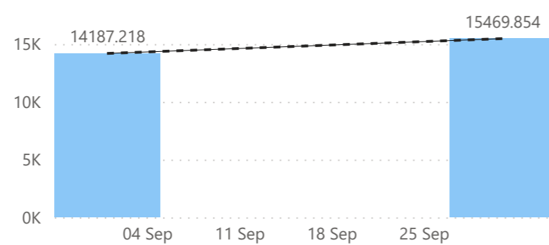
OneDrive Storage
