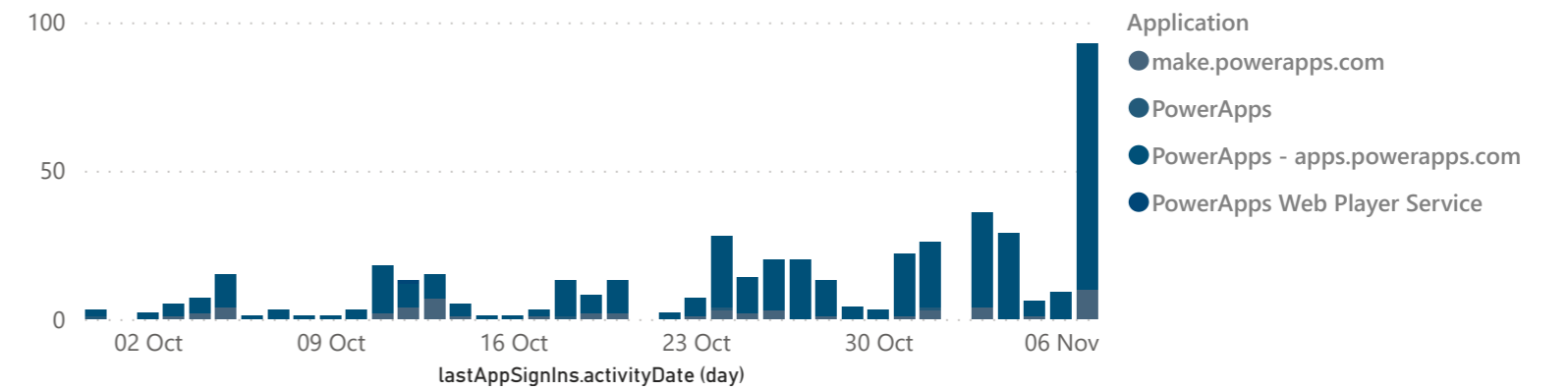
PowerApps Activity
